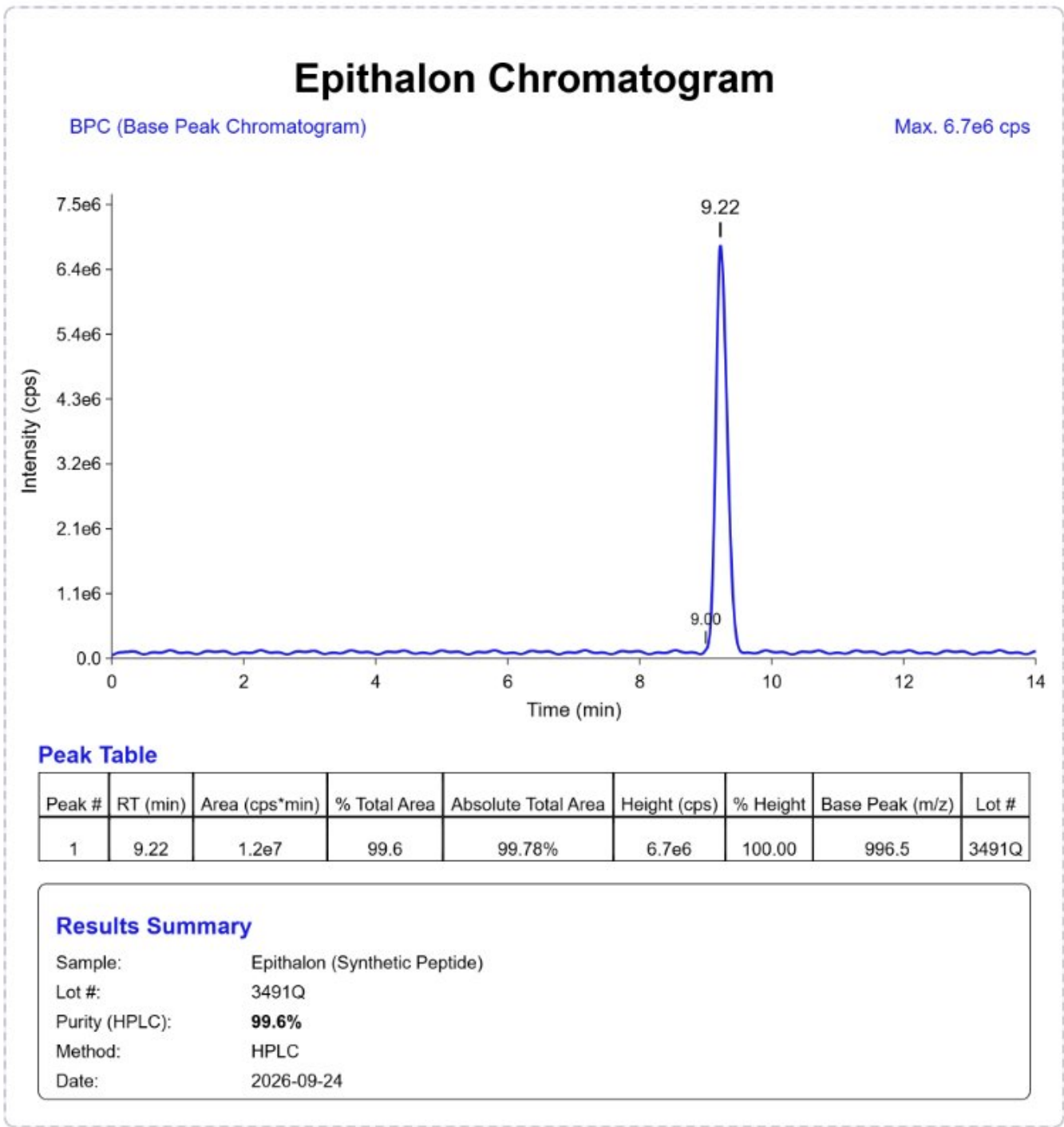
HPLC CHROMATOGRAM
