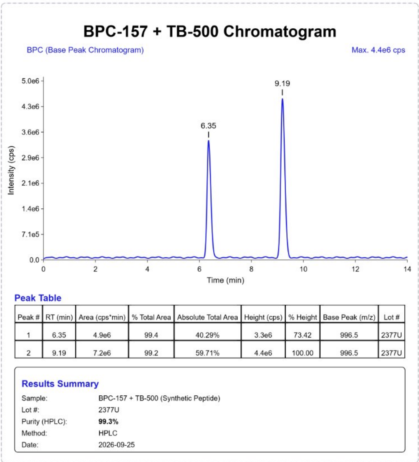
HPLC CHROMATOGRAM
