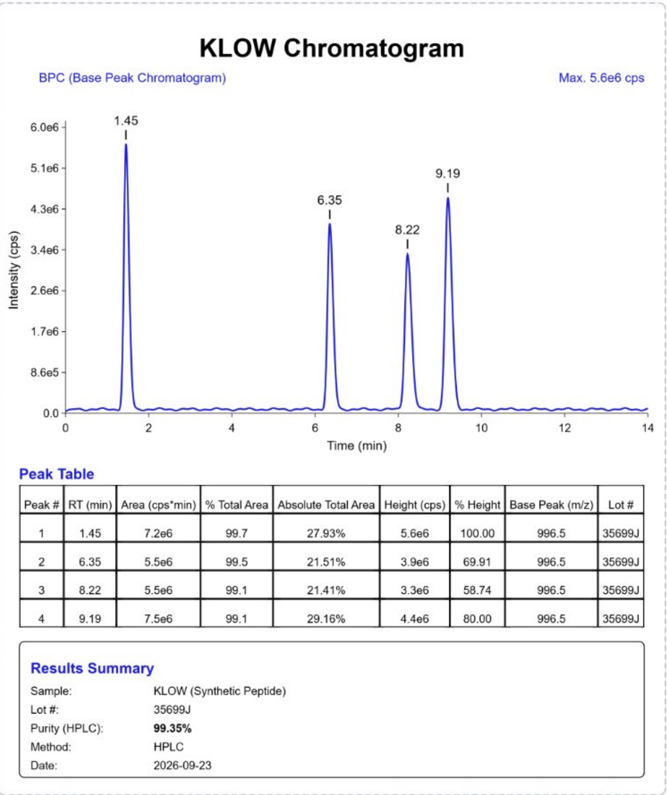
HPLC CHROMATOGRAM
