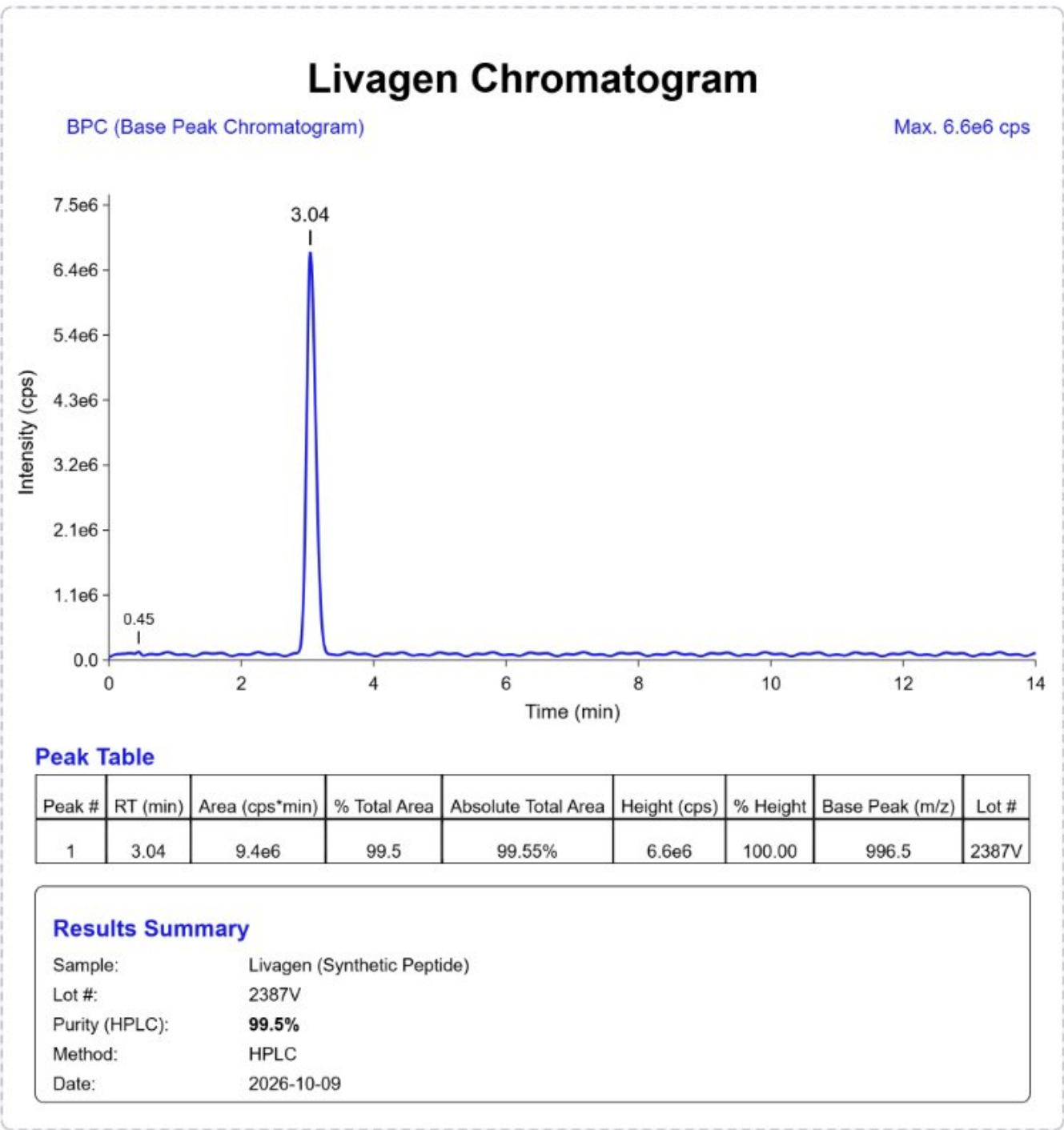
HPLC CHROMATOGRAM
