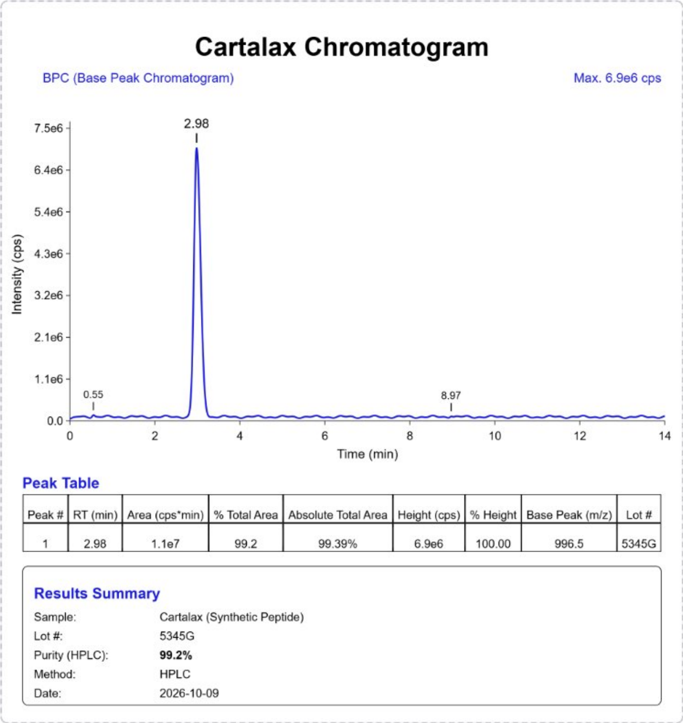
HPLC CHROMATOGRAM
